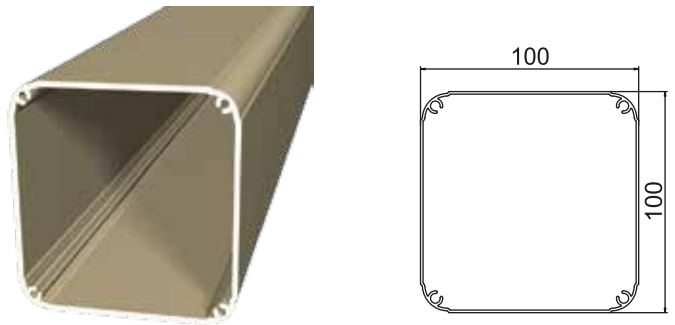
Column 100x100 mm
